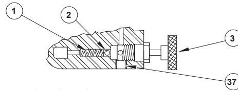
SECTION 'D-D'
